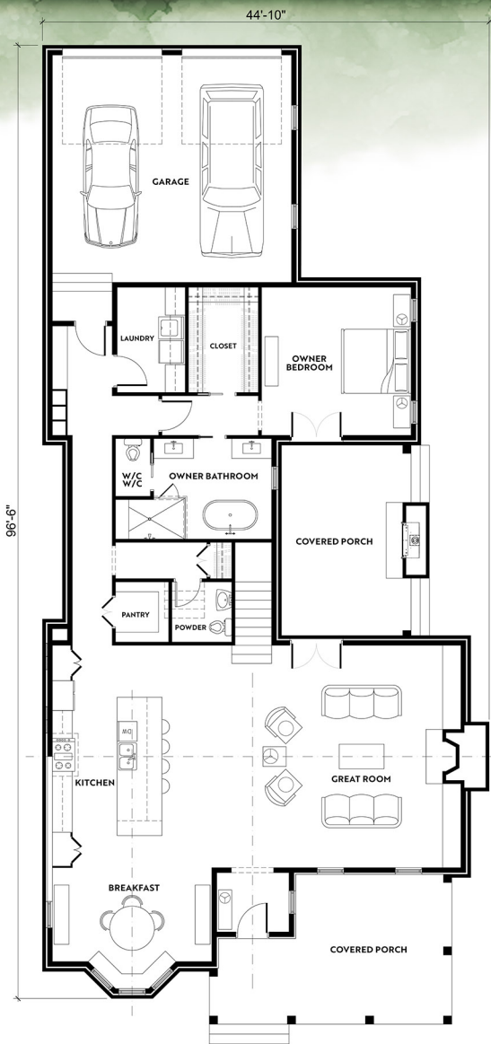
FIRST FLOOR - 2,200 SQ. FT.
