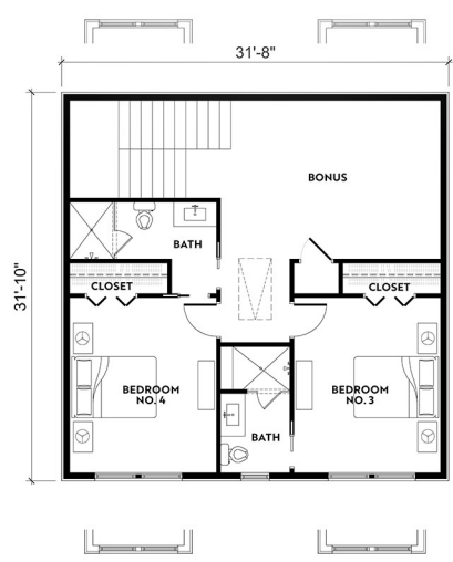
SECOND FLOOR - 897 SQ. FT.
